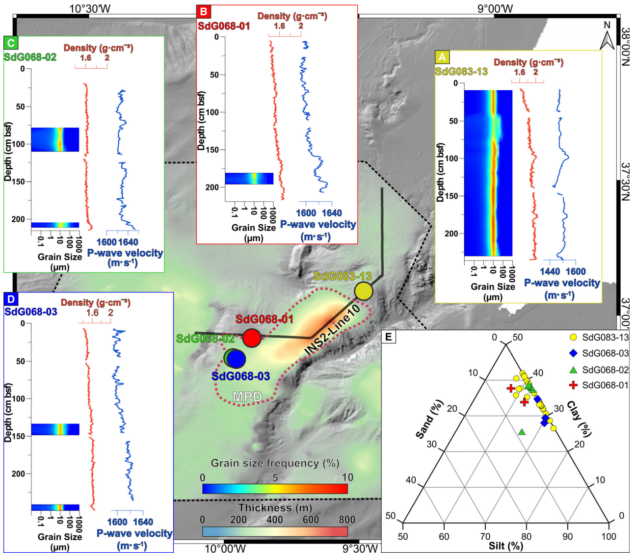
Fig. 7. Location, grain-size distribution, multi-sensor core logger (MSCL) gamma ray densities (red lines) and P-wave velocities (blue lines) of gravity cores collected for this study plotted with Unit IV thickness distribution. Red dashed outline shows the approximate areal distribution of the Marquês de Pombal Drift (MPD). (A) SdG083-13, yellow circle; (B) SdG068-01, red circle; (C) SdG068-02, green circle; (D) SdG068-03, blue circle. (E): Ternary diagram showing percentages of sand, silt and clay components for the different cores.
