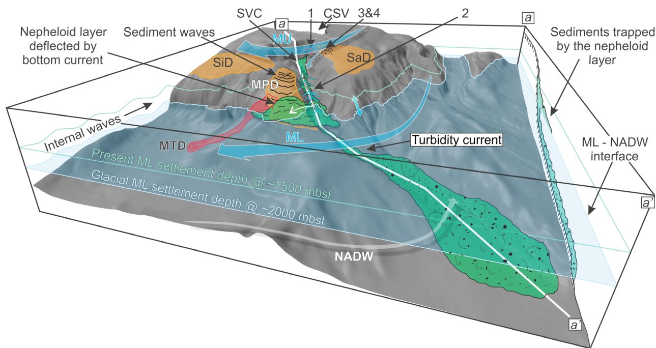
Fig. 8. Schematic representation of potential types of indirect interaction between the Mediterranean Outflow Water (MOW) and the sediment travelling along the São Vicente Canyon displayed during a glacial period. 1: Classical turbidity currents; 2: internal waves trapped in the canyon inducing sediment resuspension; 3: the denser lower part of the MOW upper core (MU) sinks in the canyon and rejoins ML at its neutral buoyancy level; 4: the MU entrains sediment in suspension, the near-bed water column gains density and sinks in the canyon. All of the scenarios require the formation of a nepheloid layer between the MOW and NADW along which the sediment finer fraction detached from the bottom of the canyon is incorporated in the MOW lower core (ML). White line along a–a' displays 2D section of sediment gravity flow and intermediate nepheloid layer on the side of the block diagram. CSV: Cape São Vicente; MPD: Marquês de Pombal Drift; SaD: Sagres Drift; SiD: Sines Drift; SVC: São Vicente Canyon; MU: MOW upper core; ML: MOW lower core; NADW: North Atlantic Deep Waters.
