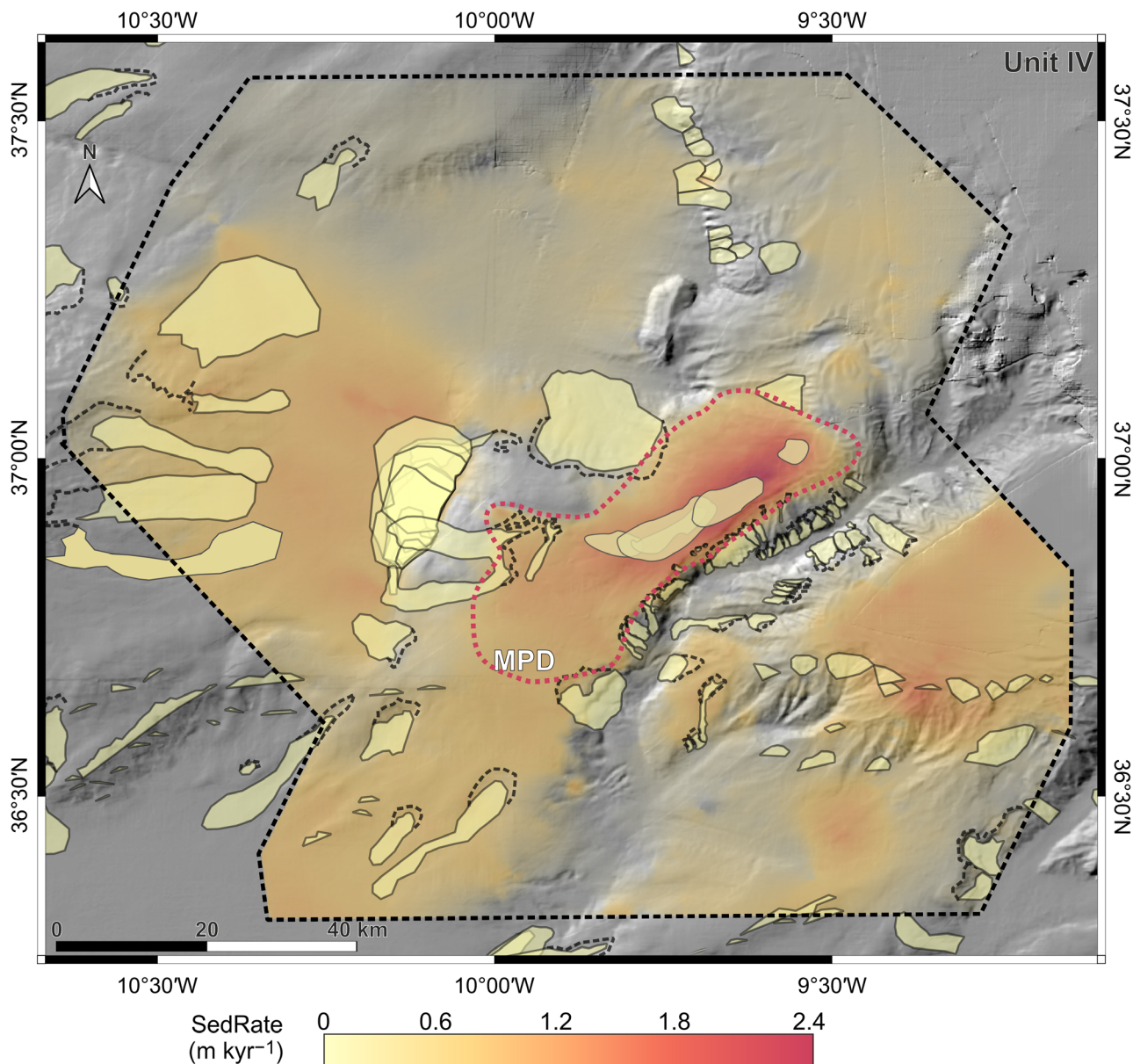
Fig. 10. Location and size of mass transport deposits (MTDs) and scars within the area of interest plotted together with sedimentation rates of the Late Quaternary Unit IV. Red dashed outline shows the approximate areal distribution of the Marquês de Pombal Drift (MPD).
