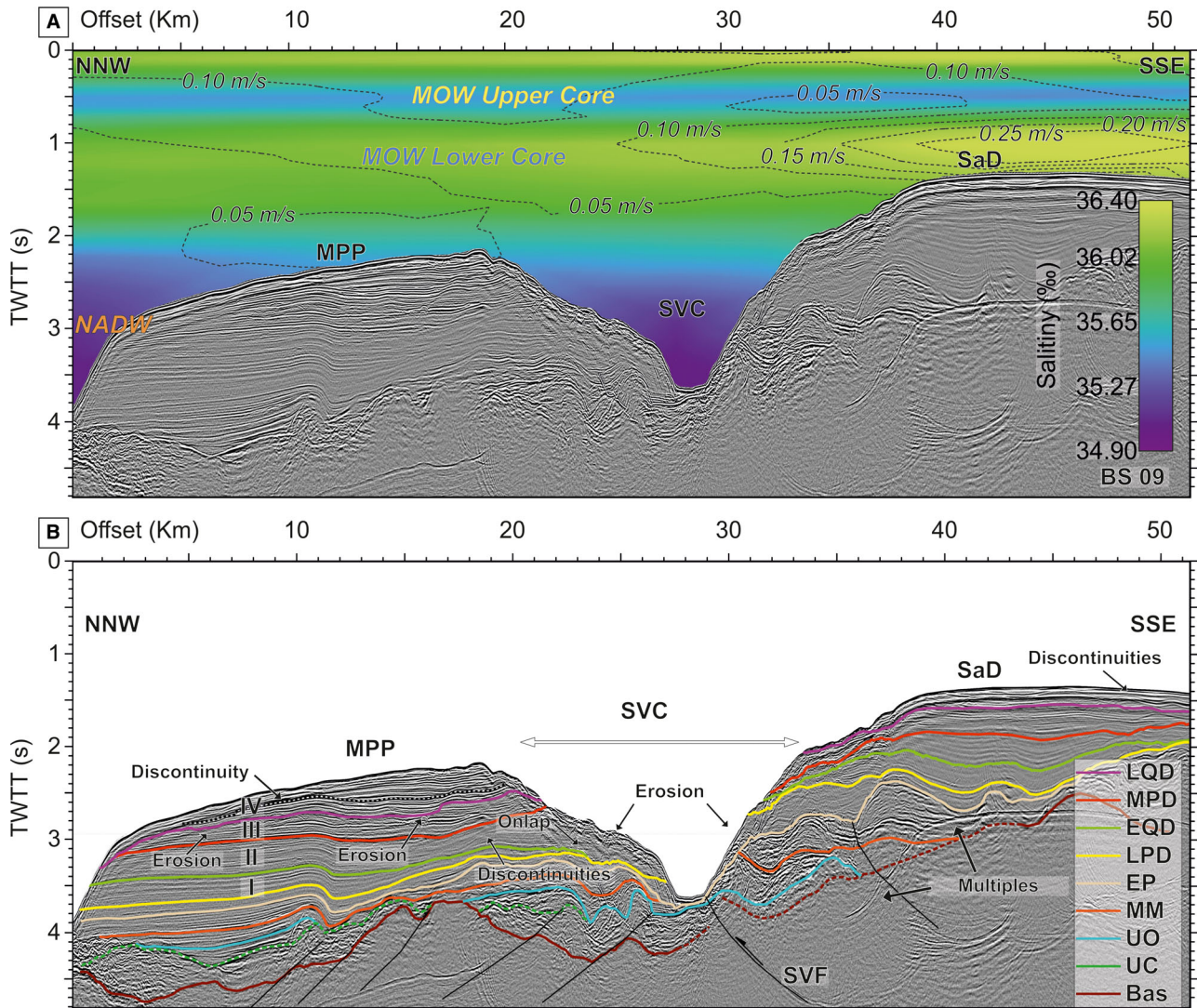
Fig. 4. (A) Uninterpreted multi-channel seismic (MCS) profile BS09 (see location in Fig. 1) with associated water salinity values (colour scale). Dashed grey contours indicate the computed water speed (Sotillo et al. , 2015; Amo et al. , 2020). (B) Interpreted MCS profile. LPD: Stratigraphic interpretation follows criteria set by Hernández-Molina et al. (2016a) and Serra et al. , (2020). LQD: late Quaternary discontinuity (0.4 to 0.3 Ma); MPD: middle Pleistocene discontinuity (0.8 Ma); EQD: early Quaternary discontinuity (2.4 to 2.1 Ma); LPD: late Pliocene discontinuity (3.2 to 3.0 Ma); EP: early Pliocene; MM: middle Miocene; UO: upper Oligocene; UC: upper Cretaceous; Bas: Basement. Orange bodies are mass transport deposits (MTDs). I, II, III and IV correspond to the different units defined in between the major discontinuities; Bas: Basement; MPP: Marquês de Pombal Plateau; SaD: Sagres Drift; SVC: São Vicente Canyon; SVF: São Vicente Fault; vertical exaggeration ca 4; TWTT : two-way travel time.
