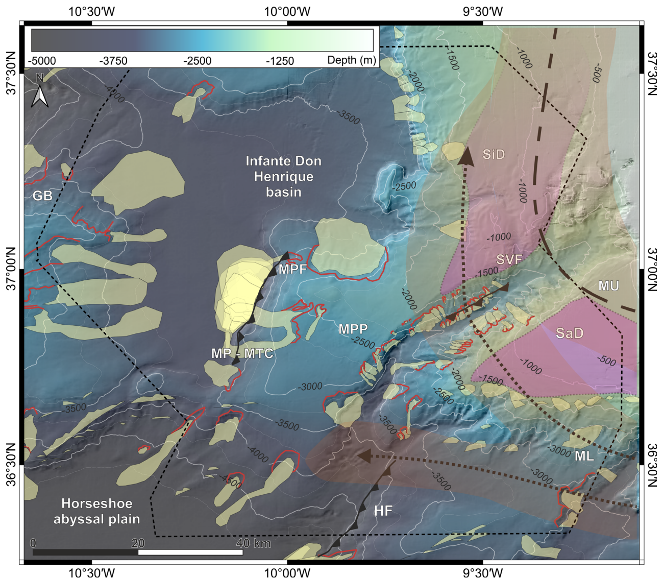
Fig. 2. Distribution of mass transport deposits (MTDs) (yellow outlines) and scars (red lines) within the area of study (dashed black outline). Dashed lines correspond to the main branches of the Mediterranean Outflow Water (MOW), with areas of influence highlighted in red. Purple areas are the estimated drift extensions. GB: Gorringe Bank; HF: Horseshoe Fault; MPF: Marquês de Pombal Fault; MPP: Marquês de Pombal Plateau; MP – MTC: Marquês de Pombal Mass Transport Complex; MU: MOW upper core; ML: MOW lower core; SaD: Sagres Drift; SiD: Sines Drift; SVF: São Vicente Fault.
