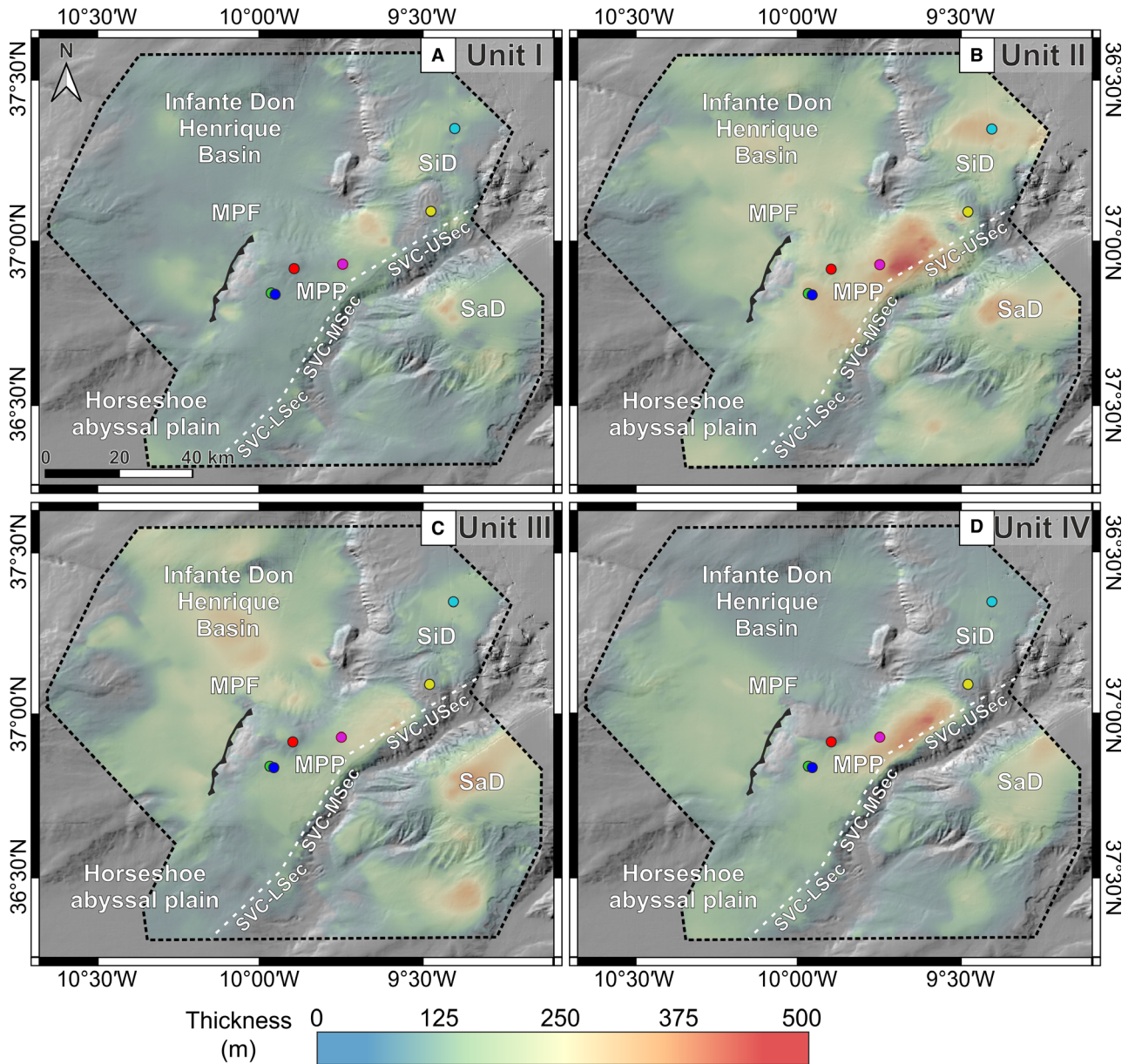
Fig. 5. Thickness distribution maps. (A) Unit I; (B) Unit II; (C) Unit III; (D) Unit IV. MPF – Marquês de Pombal Fault; MPP – Marquês de Pombal Plateau; SaD – Sagres Drift; SiD – Sines Drift; SVC – LSec: São Vicente Canyon lower section; SVC – MSec: São Vicente Canyon middle section; SVC – USec: São Vicente Canyon upper section; coloured dots indicate the location of IODP Site U1391 (light blue), multicore MC1 (red) and gravity cores SdG083-13 (yellow), SdG068-01 (red), SdG068-03 (blue) and SdG068-02 (green).
