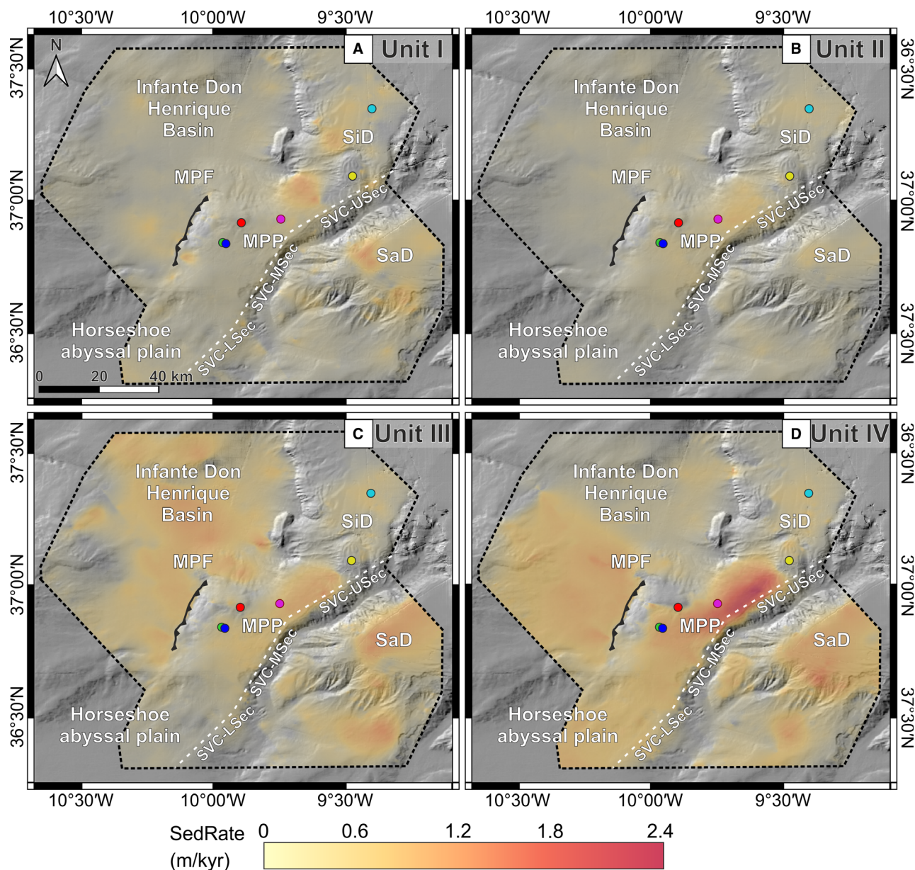
Fig. 6. Decompacked sedimentation rate maps. (A) Unit I; (B) Unit II; (C) Unit III; (D) Unit IV. MPF – Marquês de Pombal Fault; MPP – Marquês de Pombal Plateau; SaD – Sagres Drift; SiD – Sines Drift; SVC – LSec: São Vicente Canyon lower section; SVC – MSec: São Vicente Canyon middle section; SVC – USec: São Vicente Canyon upper section; coloured dots indicate the location of IODP Site U1391 and gravity cores (see Fig. 5 caption for key to colors).
