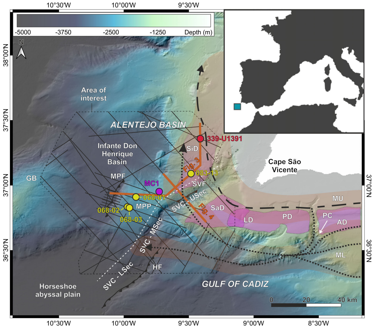
Fig. 1. Bathymetric map of Alentejo Basin and the northern part of the Gulf of Cadiz showing its main geomorphological features. Dashed arrows correspond to the main cores of the Mediterranean Outflow Water (MOW), with areas of influence shaded in red. Black lines indicate multichannel seismic (MCS) profiles used in this study. The red circle corresponds to the IODP Site U1391. Yellow circles refer to gravity cores collected during the INSIGHT Leg1 and Leg2 cruises: SdG083-13, SdG068-01, SdG068-02 and SdG068-03. The purple circle corresponds to multicore MC1 from Garcia-Orellana et al. (2006). Orange lines show the MCS profiles displayed in this paper (BS09 and INS2-Line10). Purple areas refer to the estimated drift depositional areas. The dashed polygon bounds the area of this study. AD: Albuera Drift; GB: Goringe Bank; HF: Horseshoe Fault; LD: Lagos Drift; MPF: Marquês de Pombal Fault; MPP: Marquês de Pombal Plateau; MU: MOW upper core (dashed arrow); ML: MOW lower core (dotted arrow); PC: Portimão Canyon; PD: Portimão Drift; SaD: Sagres Drift; SiD: Sines Drift; SVC - LSec: São Vicente Canyon lower section; SVC - MSec: São Vicente Canyon middle section; SVC - USec: São Vicente Canyon upper section; SVF: São Vicente Fault.
