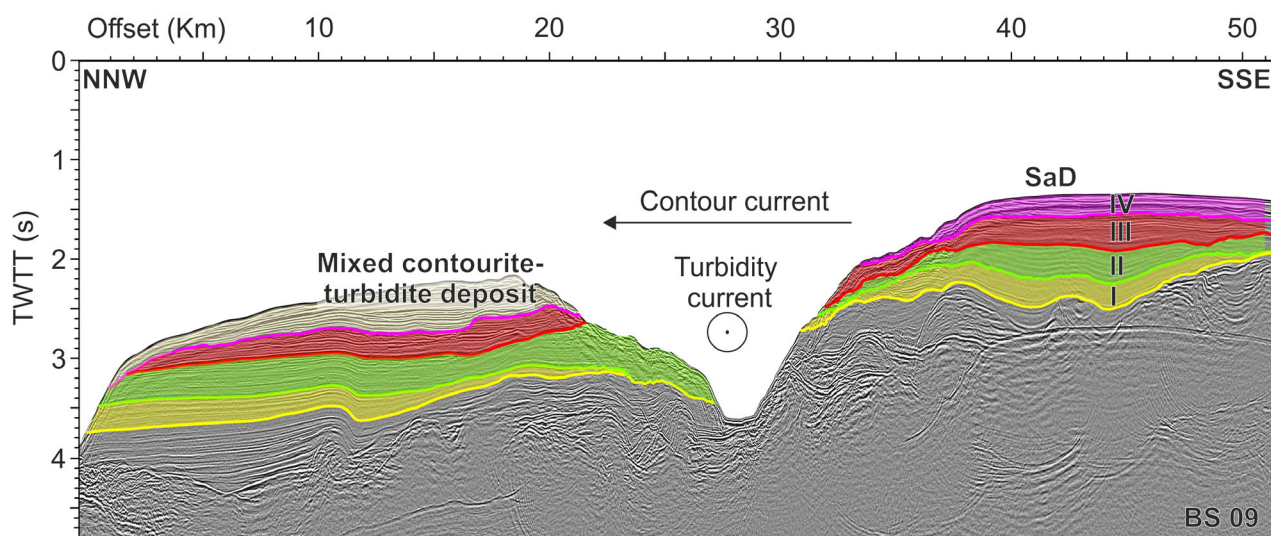
Fig. 9. Interpreted cross-section of the São Vicente Canyon from multi-channel seismic profile BS09 (see location in Fig. 1) showing position and size of the drift deposit generated by the mixed turbidite – contourite system. I, II, III and IV correspond to the different units defined in this study; SaD: Sagres Drift; SVC: São Vicente Canyon; vertical exaggeration ca 4; TWTT: two-way travel time.
